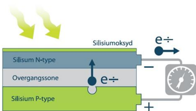
Figur 6 Prinsippkisse for solcelle [10]
